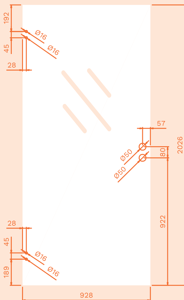
KYM 1000x2100 mm.
