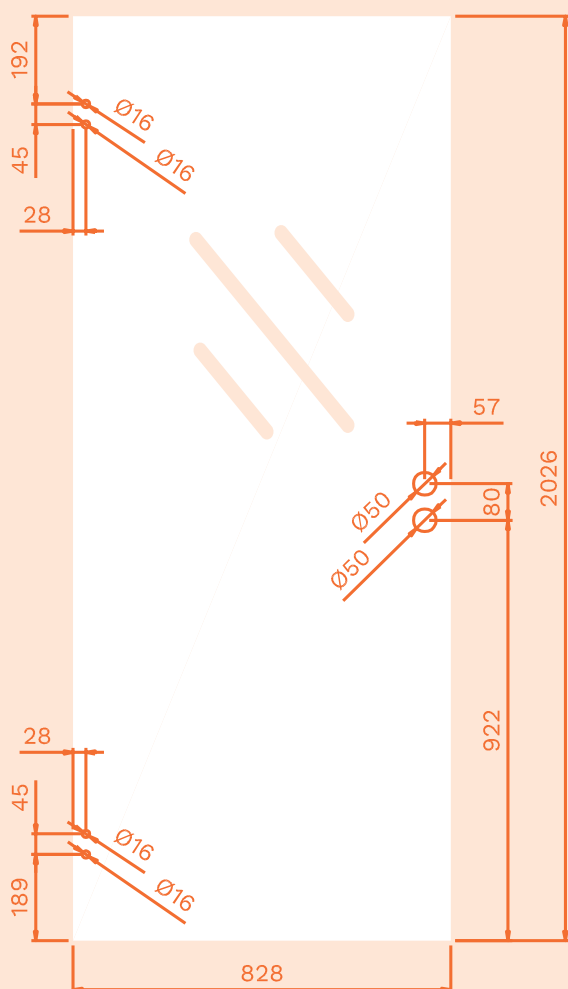
KYM 900x2100 mm.
