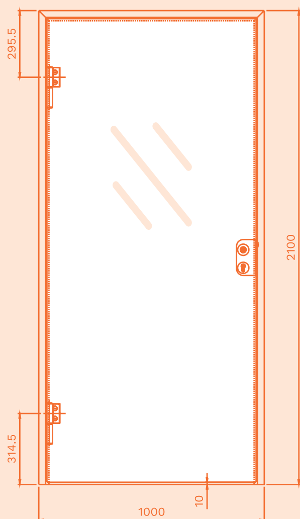
KYM 900x2100 mm.
